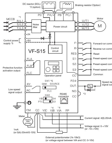
Standard connection diagram - SINK (Negative) (common:CC)
