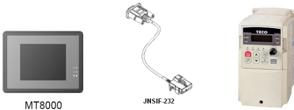
JNSIF-232Wiring Diagram:
